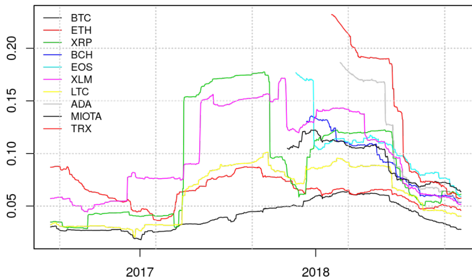
Figure 1: Volatilities of daily returns in rolling windows of 180 days length for major crypto-currencies for the time period as of 2016 until 2018-11-01. Both time-series instability as well as the sizable impact of outliers are clearly visible.
